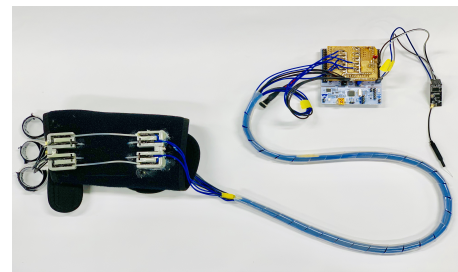
Figure 2: The glove ShareHaptics prototype: Shape Memory Alloy for actuation connected to an STM32 Nucleo-64 board.
